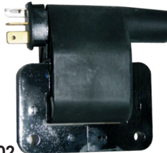
MAZDA FWD 1.6, 2.0 & FORD RANGER 2.6 (C/C 85°C - 80°C) 3 PIN
