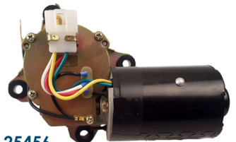
WIPER MOTOR TOYOTA COROLLA & HILUX (AE80 - AE82)
