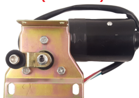
WIPER MOTOR MAHINDRA SCORPIO (12V- 50W)
