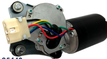
WIPER MOTOR FORD LASER & MAZDA 323 (P3) & RUSTLER
